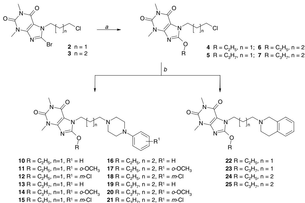
Scheme 1. Reagents and conditions: (a) RONa , ROH , reflux; (b) 1-aryl-piperazine or 1,2,3,4-tetrahydroisoquinoline, n - PrOH , K_2CO_3 , reflux.
